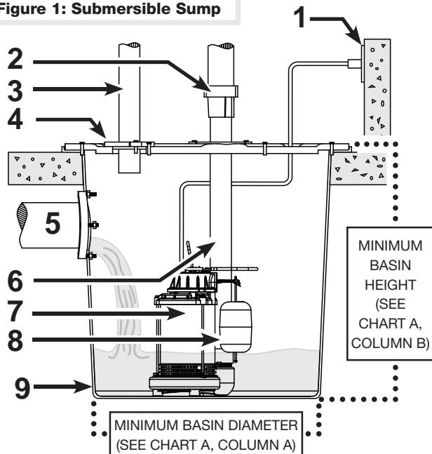
Figure 1: Submersible Sump
