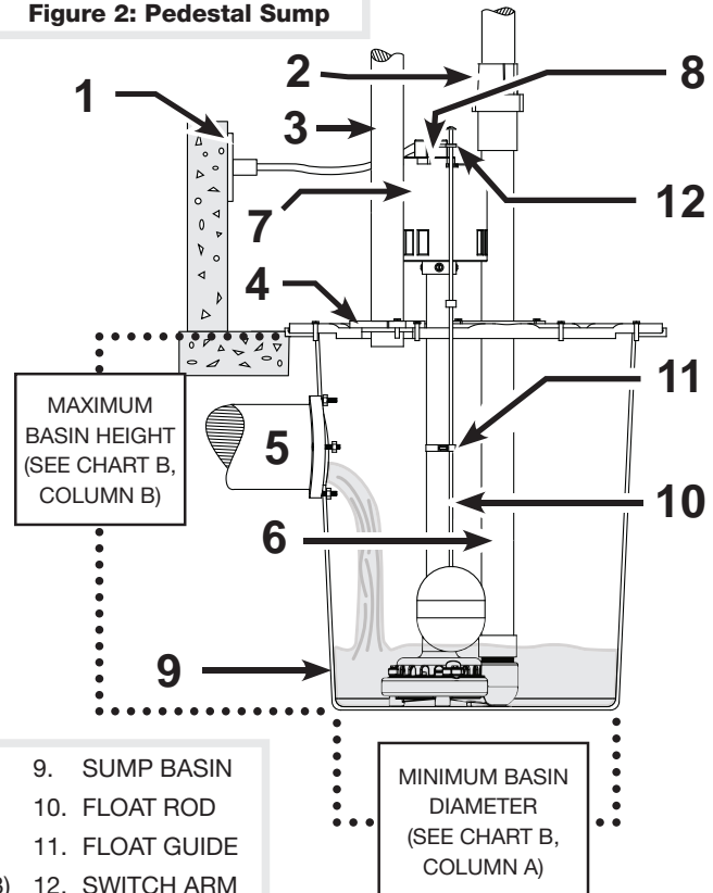
Figure 2: Pedestal Sump
